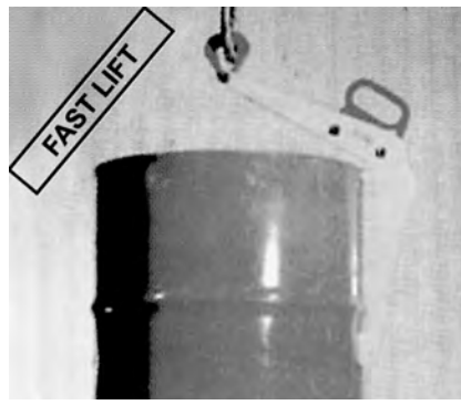
Drum Lifting Clamps
